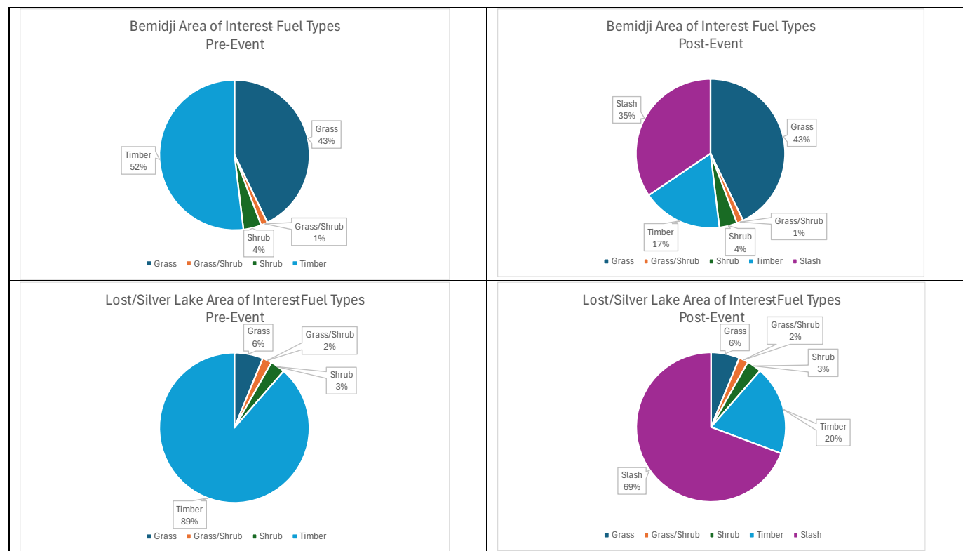
Figure 2 Change from Normal for Areas of Interest
